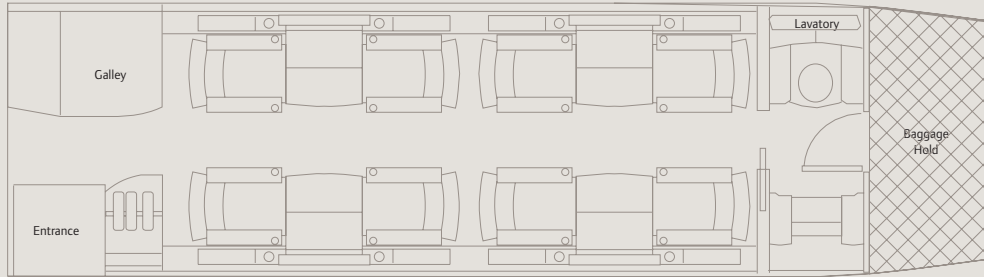
CHALLENGER 350 CABIN CONFIGURATION
